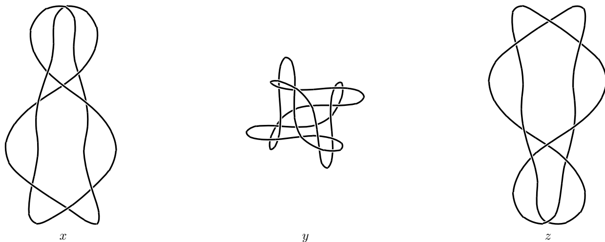
Relaxed 8_3 knot viewed along principal axes.
