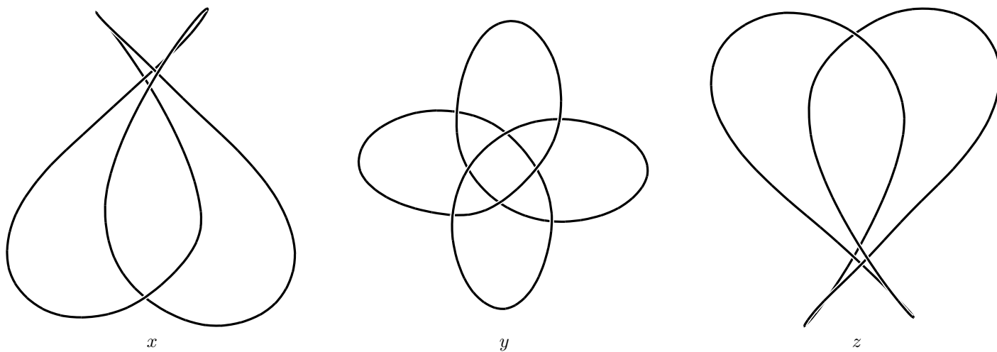
Relaxed figure-eight knot viewed along principal axes.
