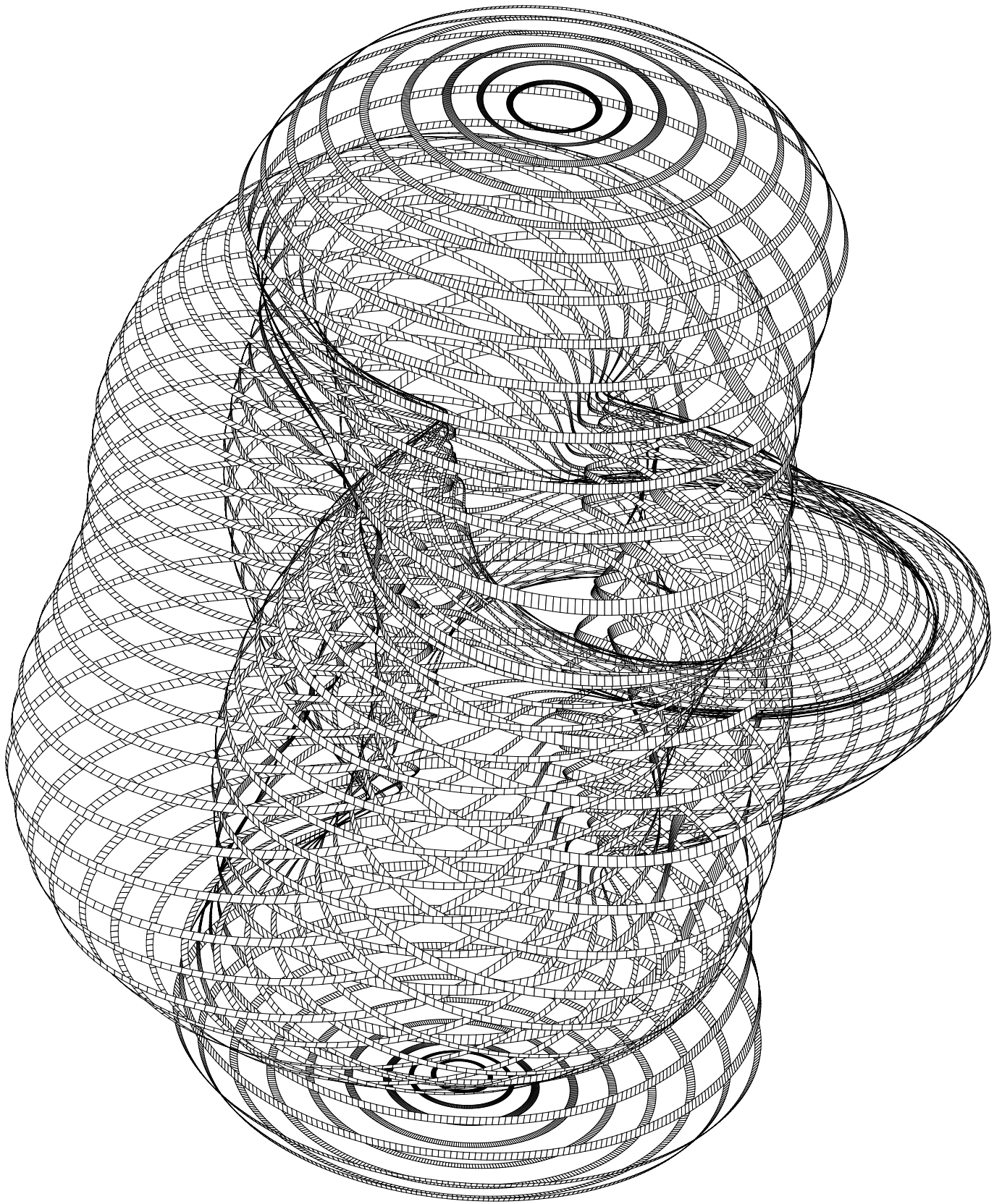
Projection of a +2-twist spun trefoil knot. The surface has transparent bands along lines of constant latitude.
