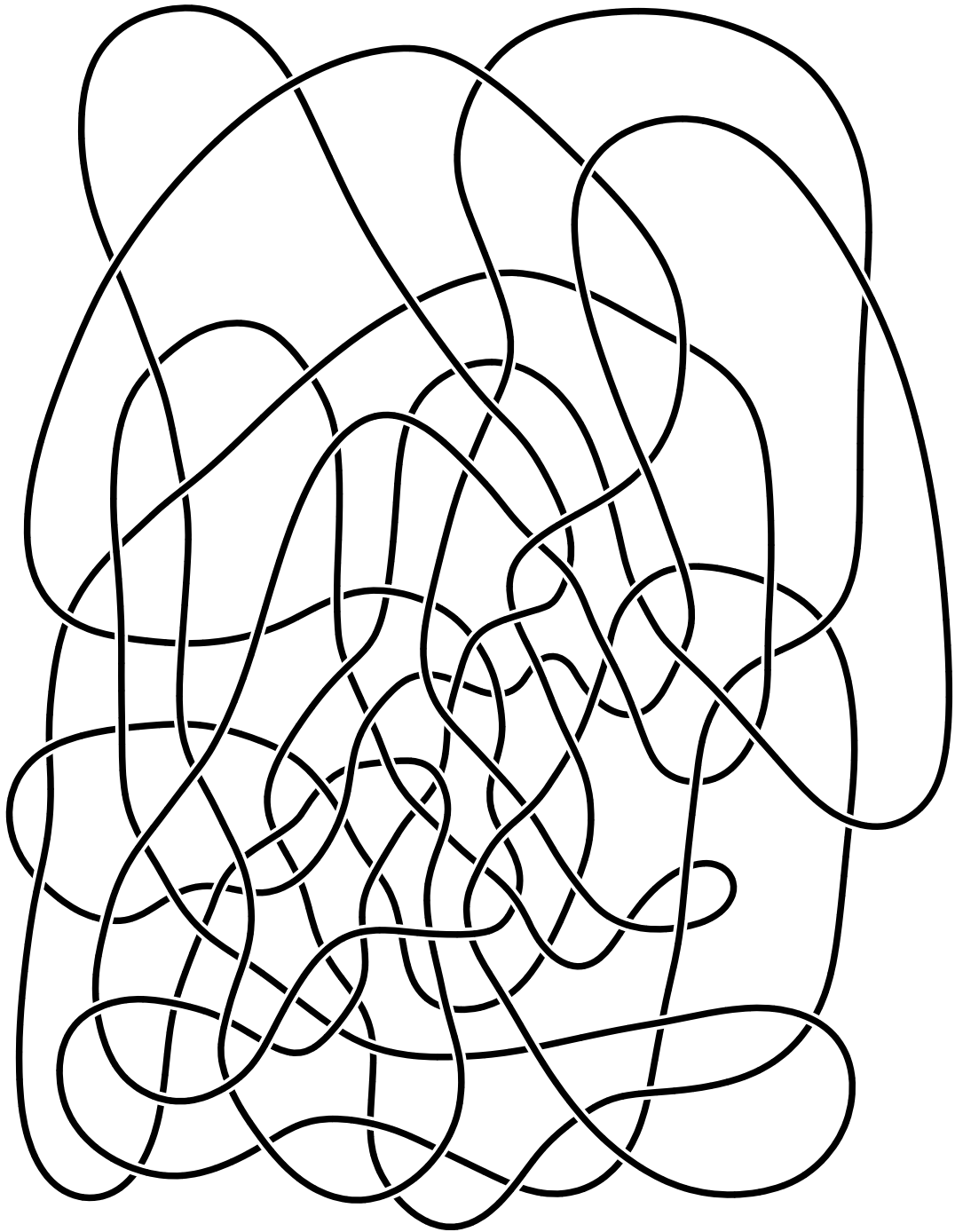
119-crossing T(2,7) knot from paper by Lewin, Gan & Bruckstein
